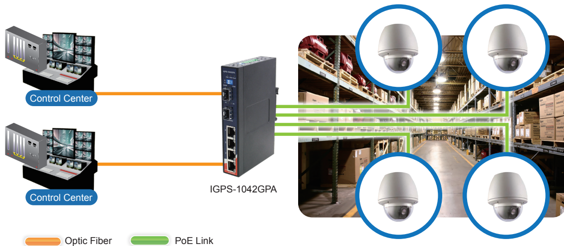
Connections of Ethernet devices
