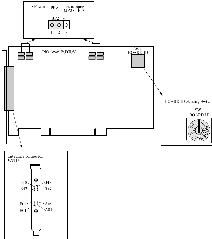
Figure 2.1. Component Locations
