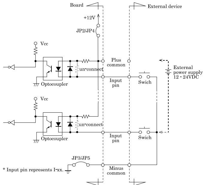
Figure 3.4. Input Circuit < PIO-32/32B(PCI)V >
