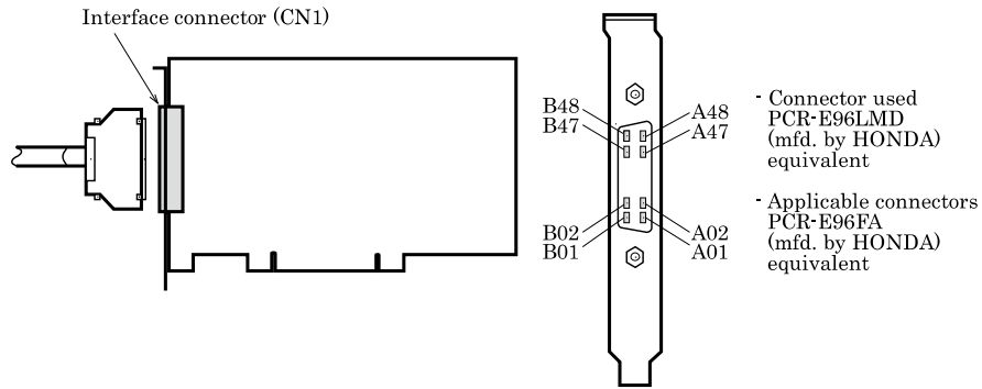
Figure 3.1. Connecting the Interface Connector
