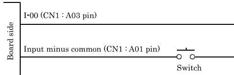
Figure 3.5. An Example to use Input I00 < PIO-32/32B(PCI)V >
