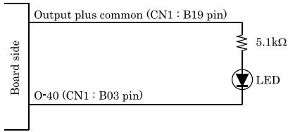
Figure 3.7. An Example to use Output O-40 < PIO-32/32B(PCI)V >
