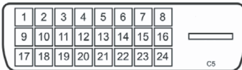
Figure 1-13: DVI-D Connector Pin Assignment
