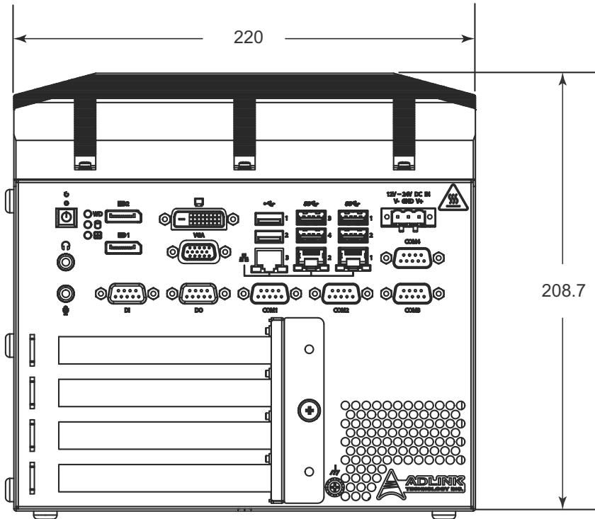
Figure 1-3: Front View
