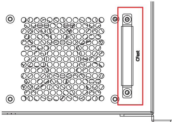
Figure 1-18: CFast Host Connector (on rear panel)
